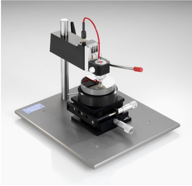
X-Y stage installed, probing 3" wafer
