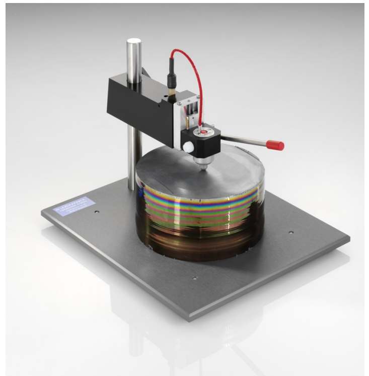
X-Y stage removed, probing ingot
