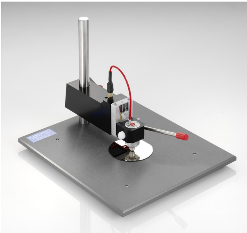
X-Y stage removed, probing 3" wafer
