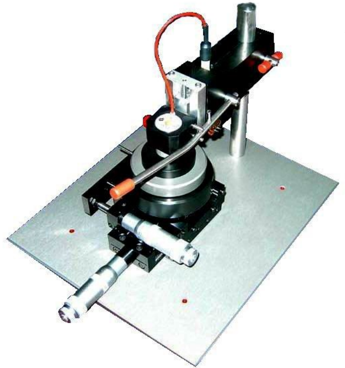
X-Y stage installed and with 2" light shield
